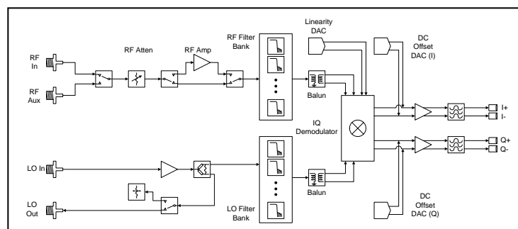
SC5313A Simplified Block Diagram
